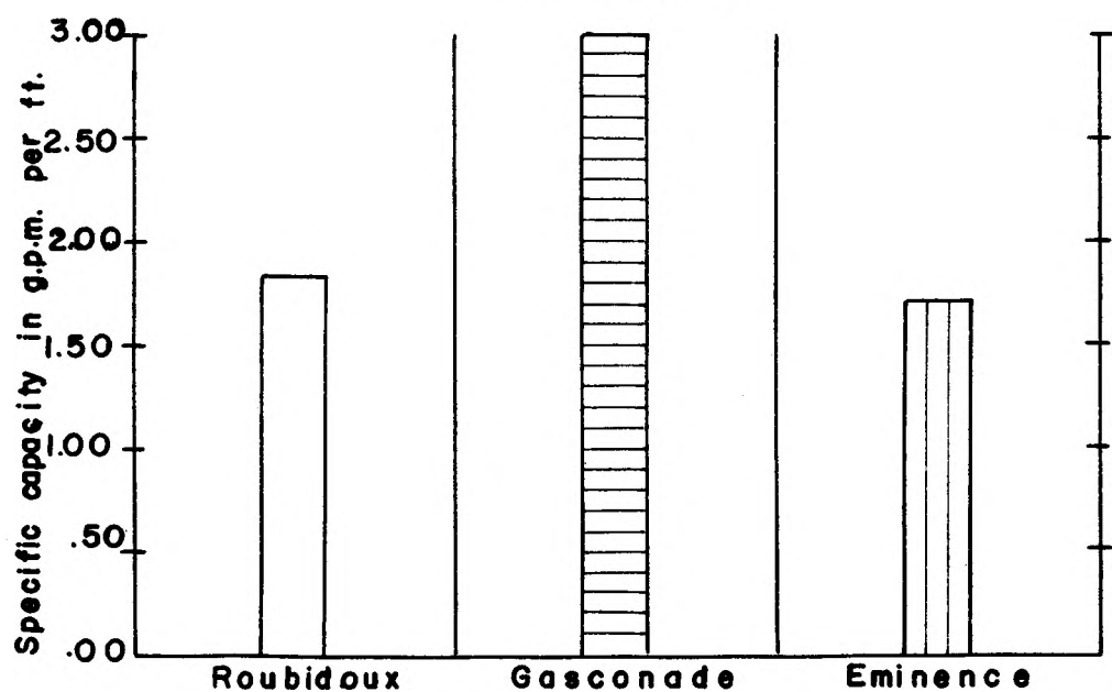
MAXIMUM SPECIFIC CAPACITY IN THE WELLS COMPLETED IN THE RB., GC., AND EM. FM.
