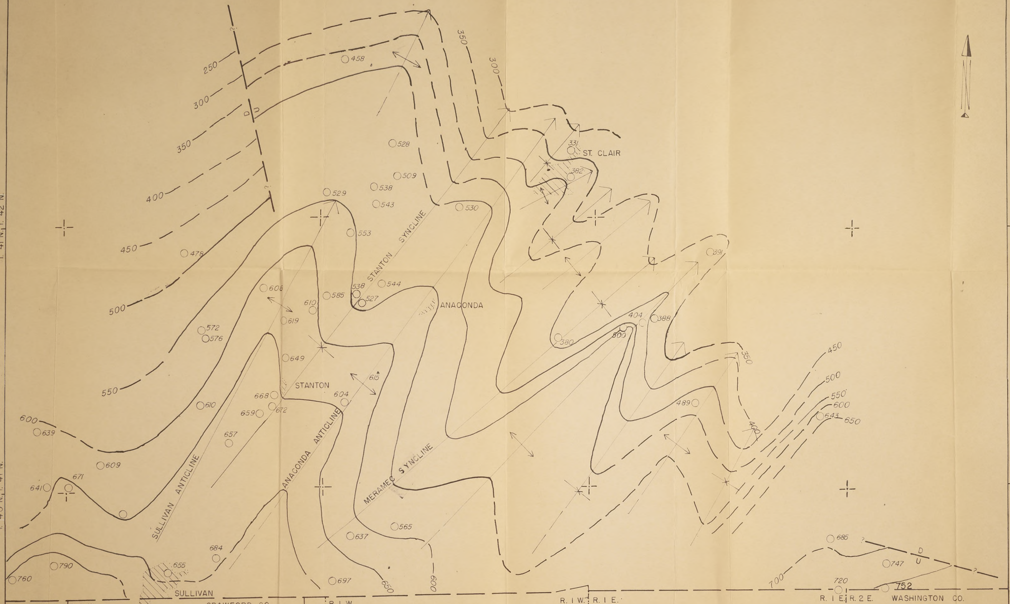
STRUCTURE CONTOUR MAP AT THE TOP OF THE EMINENCE FORMATION
